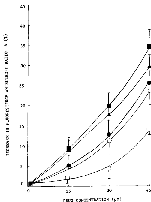
Fig. 2. Concentration-dependent increase in fluorescence anisotropy ratios, A , measured using DPH (1 μM) as the probe, by (●) tamoxifen, (■) 4-hydroxytamoxifen, (○) cis -tamoxifen, (□) N -desmethyltamoxifen, or (▲) 17 β-oestradiol, all in the range 0–45 μM. Results are shown as mean ± S.E.M., n = 3
